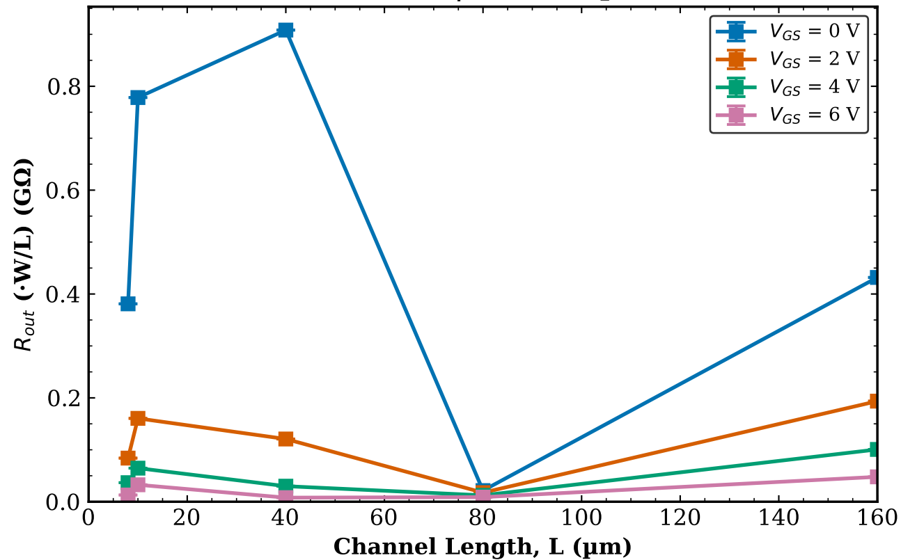
TFT1 Transistor 1 R_{out} vs L | W = 50 \mu\text{m}
